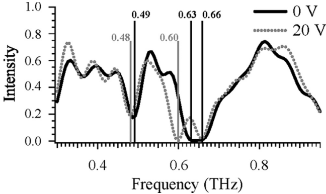
FIGURE 3 Measured reflected intensity (arbitrary units) versus frequency for a THz pulse polarised perpendicular to the slits of the sample shown in Figure 2 with 0V and 20V peak-to-peak voltages applied across the liquid crystal at a frequency of 10 kHz.
