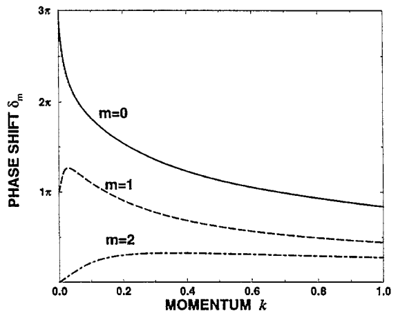
Fig. 1. Scattering phase shifts versus in-plane wave vector k (in units of inverse Bohr radius 1/a^* ) for a 2D particle in an attractive Coulomb potential screened by a 2D electron gas, screening length r_s = 1/q_s = 5a^* . Numbers show m values.
