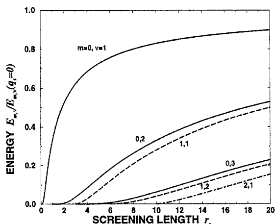
Fig. 3. The bound-state energies E_{m,\nu} plotted versus the screening length r_s for different m values. The curves are normalized by the energies for the unscreened potential, E_{m,\nu}(q_s = 0) = -(m + \nu - 1/2)^{-2} . Numbers show m and \nu values.
