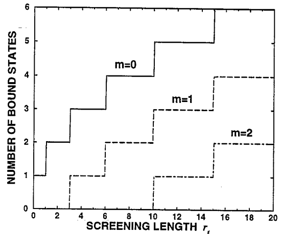
Fig. 2. Number of bound states, calculated as the low-energy limit of the phase shift, plotted versus the screening length r_s (in the units of Bohr radius a^* ). The solid line corresponds to m = 0 ; dashed line, m = 1 ; dashed-dotted line, m = 2 . New steps appear at (r_s)_c = (2m + \nu - 1)(2m + \nu)/2 , \nu = 1, 2, \dots
